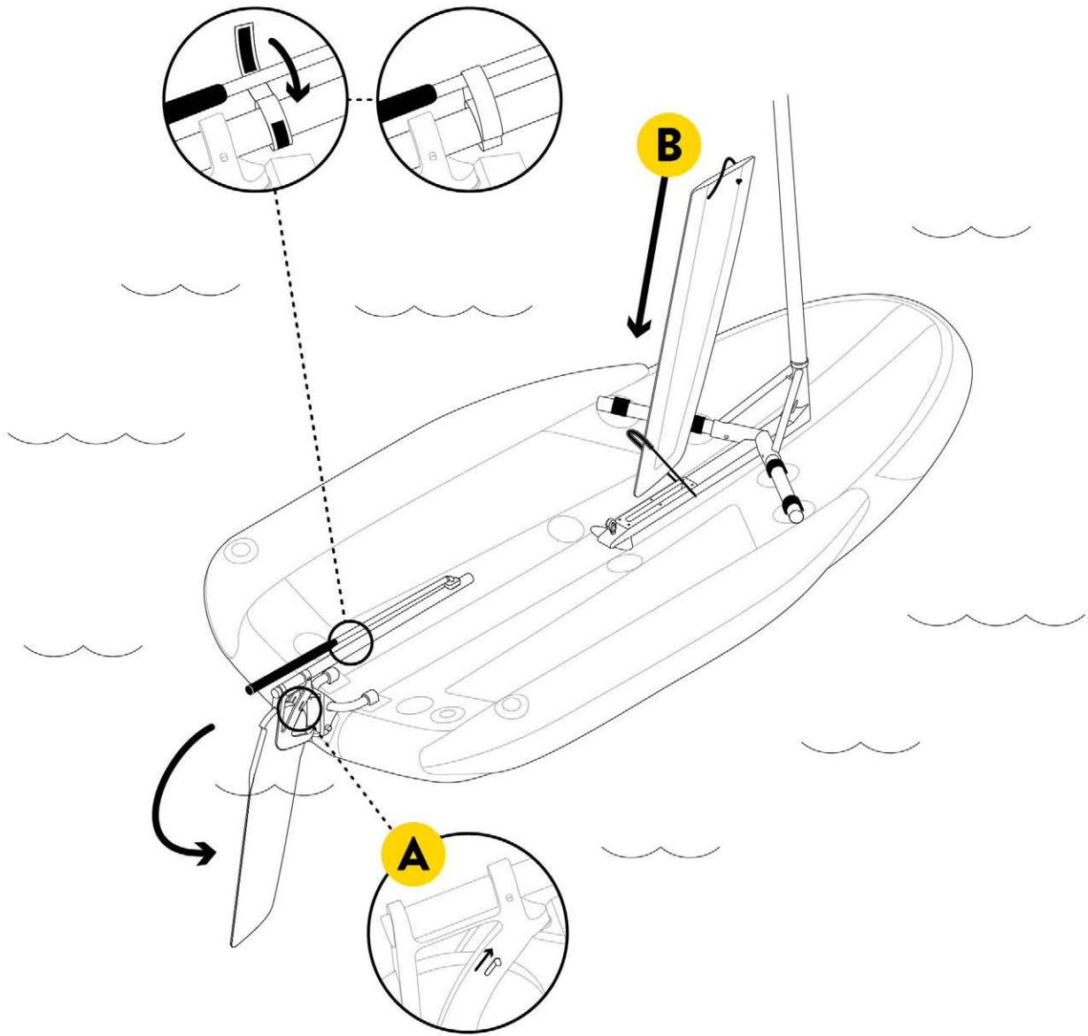
Method for attaching the tiller extension to the tiller
